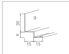
Nr. 50/22 1,0 mm dick, gelocht
