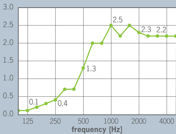
Equivalent sound absorption surface [m 2 ] OWAcoustic® vela (H = 415 mm)
