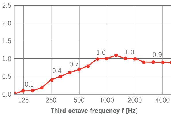
Equivalent sound absorption area [m 2 ] timber frame with printed surface (1200x800x30 mm)
