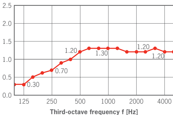
Equivalent sound absorption surface [m 2 ] Aluminium frame, inside fabric covered (687 x 1312 x 80 mm)
